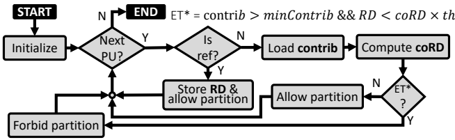
Fig. 7. Reduced Intra Sizes algorithm.
