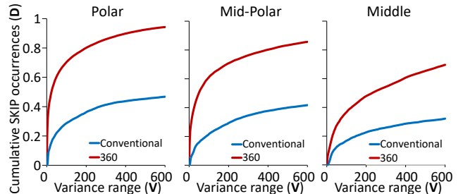
Fig. 2. Cumulative distribution of SKIP per block variance, CUs 32x32.
