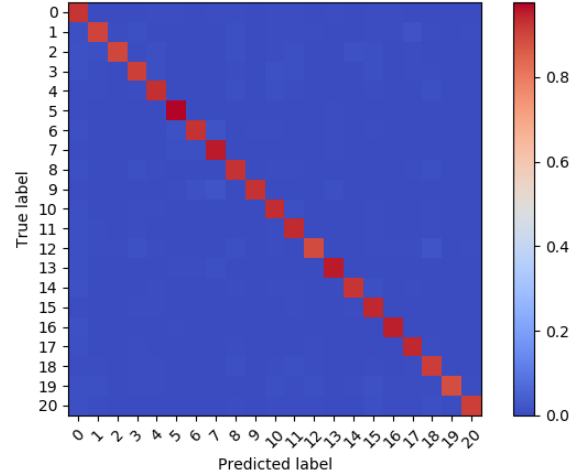
Fig. 8. Frame-level confusion matrix of MLRRN on ChaLearn Montalbano. Indexes represent different dataset classes. Class-0 represents no-gesture .
