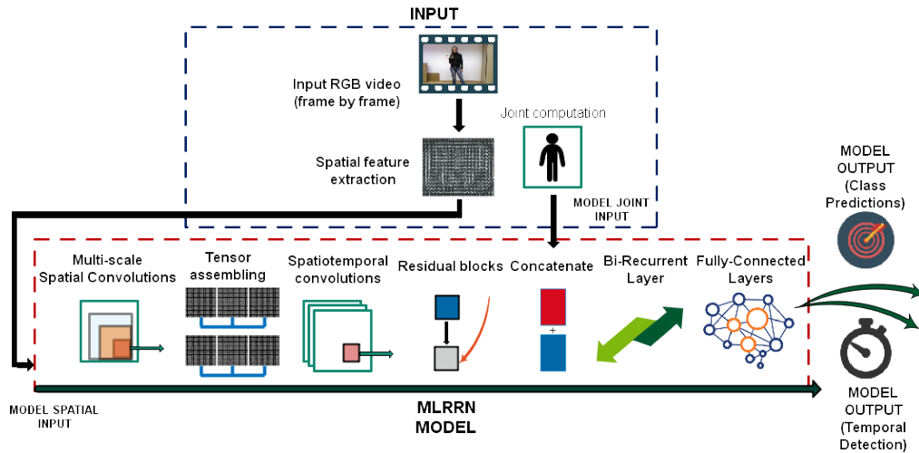
Fig. 1. Illustration of the proposed MLRRN approach.
