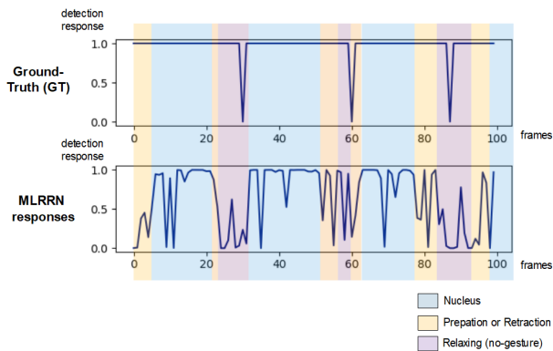
Fig. 9. Detection responses of MLRRN on ChaLearn ConGD.
