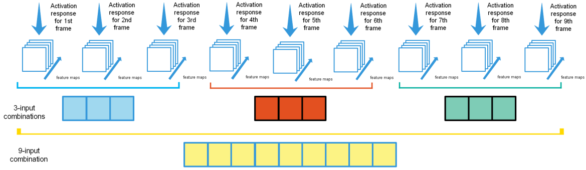
Fig. 3. Assembling of tensors on MLRRN architecture.
