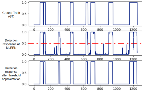
Fig. 6. Detection responses of MLRRN. Dashed red line represents the threshold used to approximate responses.
