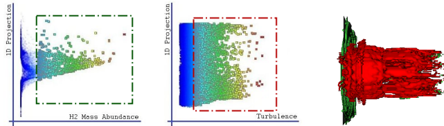
(a) Scatter Projection focused on H_2 Mass Abundance. (b) Scatter Projection focused on Turbulence. (c) Object space view of selections in (a) and (b).
