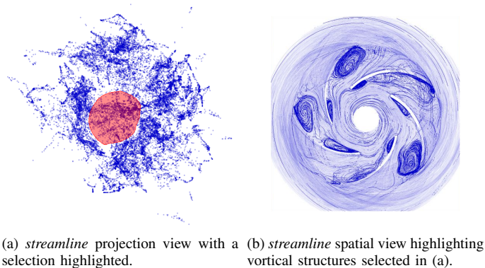
Fig. 8. TC-PLP projected layout of the streamline feature space of the Pump data and spatial view of the streamlines.
