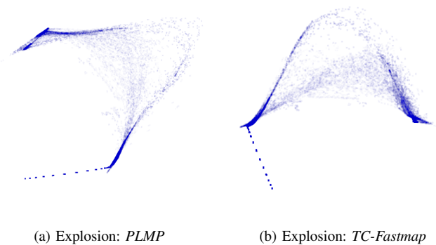
(a) Explosion: PLMP (b) Explosion: TC-Fastmap Fig. 5. PLMP and TC-Fastmap layouts of the Star Explosion data (volume 90).
