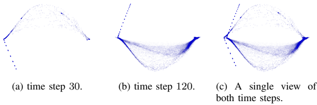
Fig. 1. Fastmap layouts relative to two distinct time steps of the ( VisContest 2008 ) simulation data. The layout obtained for time step 120 is rotated as compared with that of time step 30. The rightmost figure highlights this limitation of current projection techniques.
