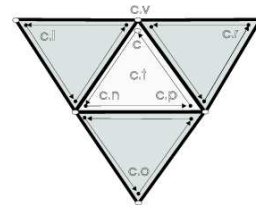
Figure 2: Corner notations.
