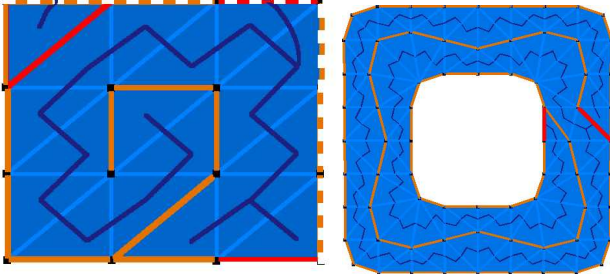
Figure 6: (left): a primal remainder on a torus (genus 1): the topmost and bottommost horizontal edges are identified, and so do the leftmost and rightmost ones. (right) a primal remainder on an annulus (two boundary curves).
