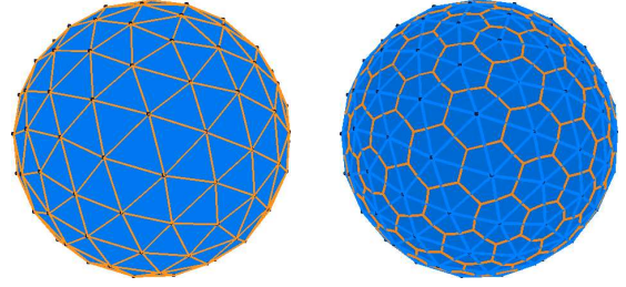
Figure 4: (left): the primal graph and (right): the dual graph of a triangulated sphere.
