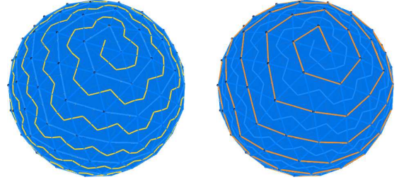
Figure 5: (left): a dual spanning tree \Theta(S) extracted from the dual graph of Figure 4(b). (right): the primal remainder \Gamma(S) of \Theta(S) , which is a subgraph of the primal graph of Figure 4(a).
