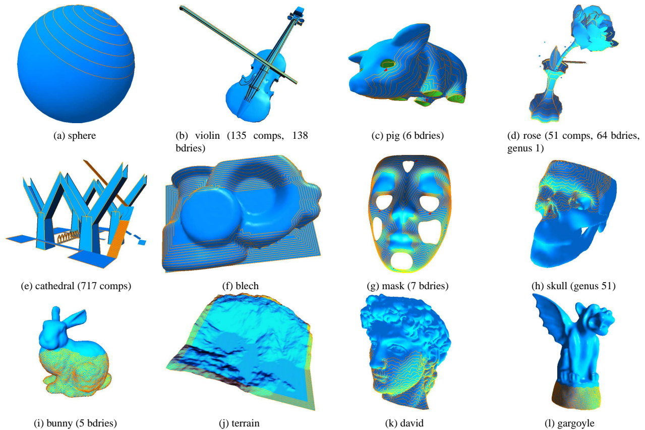
Figure 11: Some of the models used for the experiments, with the beginning of the dual spanning tree generated by Edgebreaker.
