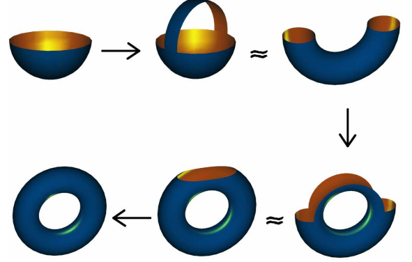
Figure 1: Handlebody decomposition of a torus [8].
