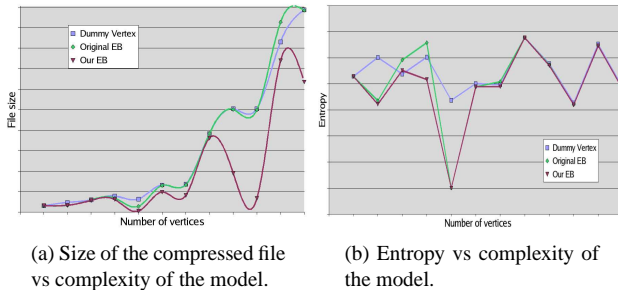
Figure 10: Comparison of the final size and of the entropy of the Edgebreaker’s symbols: for the range encoder, those parameters depends more on the regularity than on the size of the model, but our algorithm really enhance the previous results.
