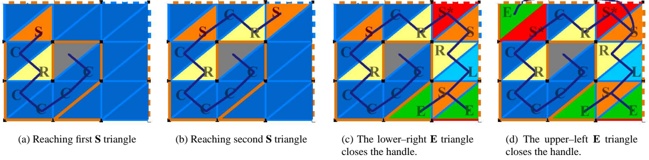
Figure 8: Coding of a torus: the creation of two handle S triangles: the first and the second S symbols.
