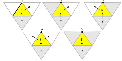
Figure 7: The Edgebreaker encoding.
