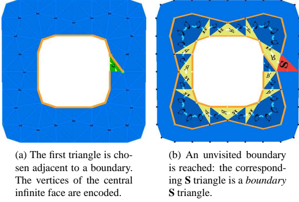
Figure 9: Coding of an annulus: initialization and creation of boundary S triangles.
