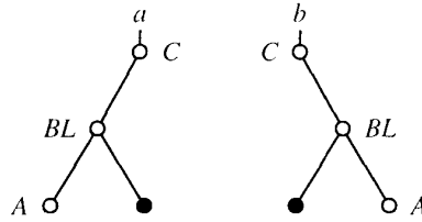
Figure 4: Trees a and b are different, but have the same depth-first order listing, ABLCA , of their nodes.
