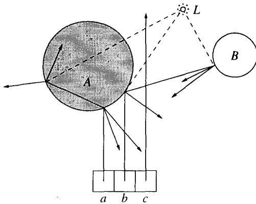
Figure 1: Paths followed by three adjacent rays a , b , and c , up to recursion depth 2 of their paths. Ray a hits sphere A where it reflects and refracts. Ray b also hits sphere A , but the angle does not permit refraction at that point. Its reflection, though, hits sphere B . Finally, ray c does not hit any object in the scene.
