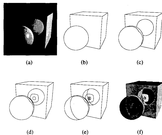
Figure 7: Different levels of detail for edge detection. (a) Original; (b) Depth 1; (c) Depth 2; (d) Depth 4; (e) Depth 6 with light visibility; (f) Segmented at depth 6 with light visibility.
