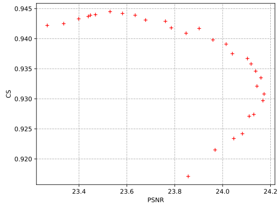
Fig. 5. Cross-plot between CS and PSNR. The correlation coefficient between CS and PSNR is -0.6591 , implying that higher values of PSNR do not always result in higher values of CS.
