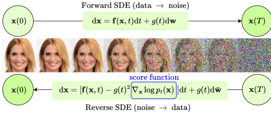
Fig. 1. Forward and reverse processes. Adapted from [15].
