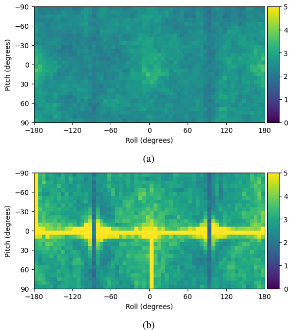
Fig. 5. Median error for each pitch/roll for VectorUp (a) and AnglesUp (b).
