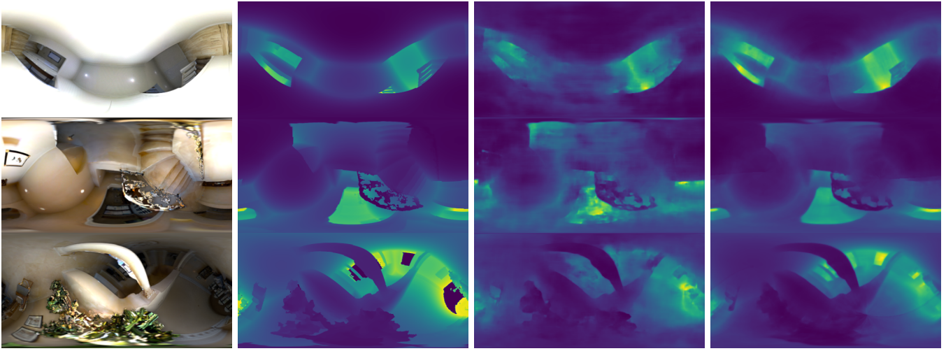
Fig. 8. Depth inference results. First column shows color images. Second to fourth columns present the ground-truth depth maps and the estimates from the baseline OmniDepth and OmniDepth when supplied with VectorUp.
