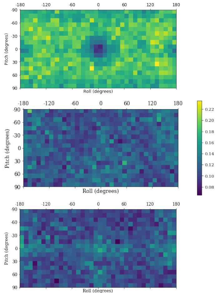
Fig. 9. Relative depth error varying the rotation angles (roll and pitch) without rotation correction (top), with VectorUp (middle) and with AnglesUp (bottom)
