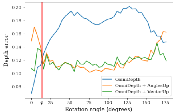
Fig. 7. Mean Absolute Relative error in depth for OmniDepth (blue) and its rotation-aware versions using VectorUp (green) and AnglesUp (orange) as a function of the angular deviation from the gravity vector. The red vertical line at \psi = 14^\circ indicates the angular threshold where rotation-aware versions improve over the baseline.
