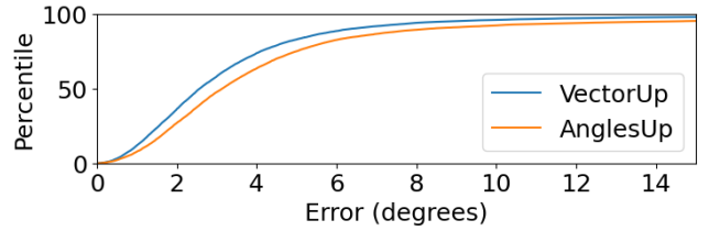
Fig. 4. Percentiles versus the angular error in degrees for VectorUp and AnglesUp.
