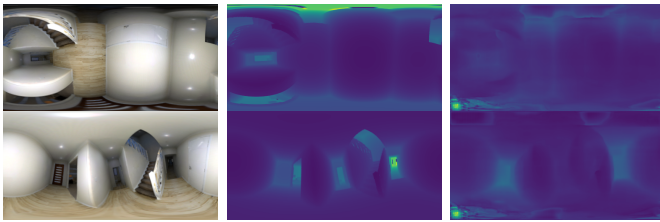
Fig. 10. Depth inference results. In the first row: rotated color and depth maps (ground-truth and results from BiFuse). In the second row: upright corrected color and depth maps (ground-truth and results from BiFuse).
