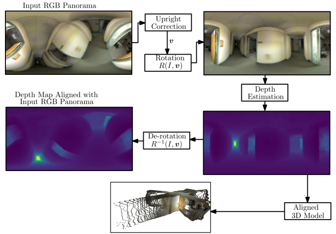
Fig. 3. Overview of our method, where R(I, \mathbf{v}) denotes the rotation of the spherical panorama I that aligns a unit vector \mathbf{v} of I with the vertical axis.
