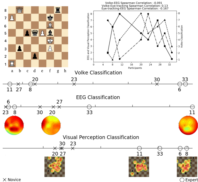
Fig. 7. (Top left) Chessboard diagram of the C4 on-screen question "May the BLACK QUEEN achieve checkmate in ONE move?". The correct answer is no; (Top right) Spearman's correlation of the degree of monotonicity between the series of paired participants ranked by the Volke and Visual Perception classifications shown as one-dimensional discriminant axes (in the middle); (Bottom) From left to right, corresponding spatial attention maps of the participants 29 (novice), 8 (expert), and 33 (expert).
