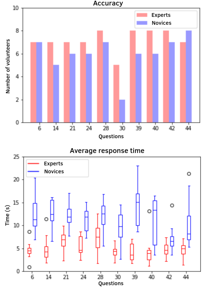
Fig. 4. (Participants' performance in Category 3.
