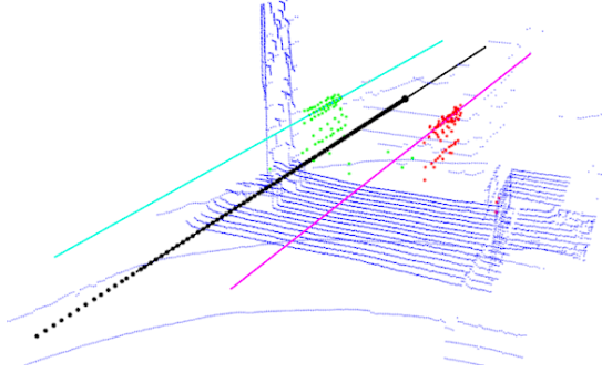
Fig. 5: Illustration of the trajectory estimation. The image shows the lines regressed for both sides of the truck (cyan and pink lines) using the set of points of the border of the bucket (green and red points respectively), as well as the average line defining the trajectory (black line).
