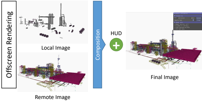
Fig. 4. Schematic representation of the two framebuffers on the client side: one for local rendering and the other for remote rendering. This separation prevents the client to redraw the local scene when a new remote image is available. Instead, the client only combines the local image with the remote image according to their respective depth values. After, the client draws the HUD elements over this combined image.
