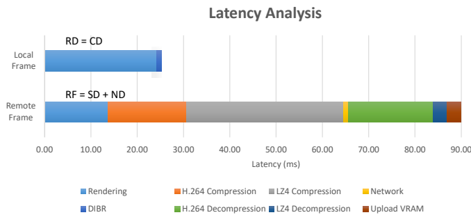
Fig. 8. The latency involved in each step of our methodology. The difference in time between the acquisition of local image and remote image clearly shows the advantage of the hybrid approach. Hence, the user has a faster response even on limited bandwidth.
