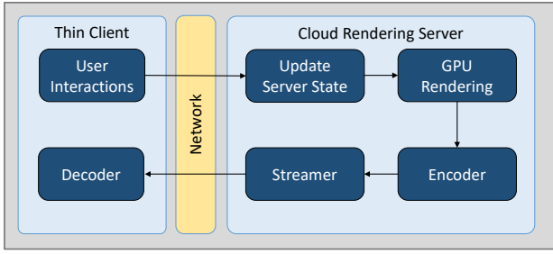
Fig. 1. The phases involved in a typical cloud rendering system
