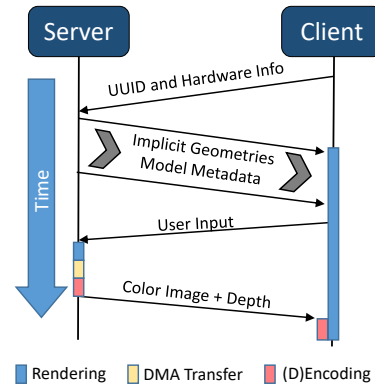
Fig. 3. The communication model between the server and the client. The first frames are displayed after the first geometries arrive on the client side.
