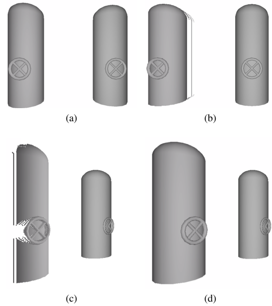
Fig. 9. Image quality comparison during the navigation on the scene. (a) is the initial view. (b) and (c) are the results while navigating through the scene. (d) is the image completion when the user stop interacting with the scene.
