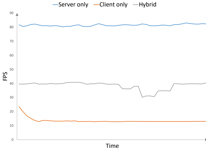
Fig. 7. Fps rate obtained using three different approaches: server only; client only and a client-server hybrid rendering. The total execution time in each test is 50 seconds.
