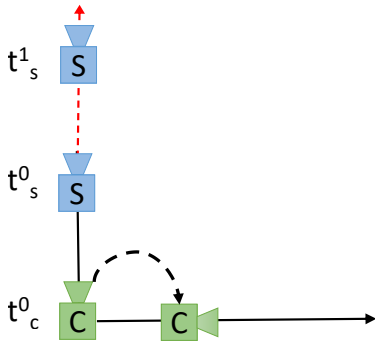
Fig. 5. Schematic representation of the lag compensation and path correction. At t^0 the server camera (the blue) is displaced relative to the client one (the green). This displacement in time as being the moving average ( ma ) of the response delay, i.e. t_s^0 = ma(RD) + t_c^0 . At t_c^0 , the user rotates the camera to the right and, after this moment, the server camera will be on invalid path (red path). The server is notified only at t_s^1 due to the uplink latency, i.e. upl = t_s^1 - t_s^0 . So, it's necessary to move the server camera back to the position at the event took place, next we execute the user event and lastly we displace the server camera again.
