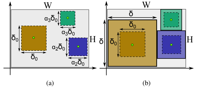
Fig. 5: (a) The input layout with \delta_0 being the length of the coarser cell. The size of the remaining cells are defined according to the initial parameter \delta_0 and their scale parameters \alpha_i . (b) The result of the optimization when \delta > \delta_0 .
