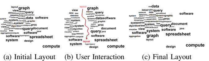
Fig. 8: Word cloud with size varying primitives
