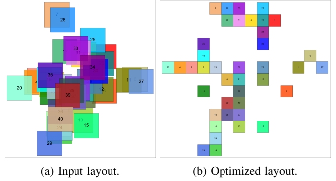
Fig. 4: Result of our method to rearrange boxes with overlaps.
