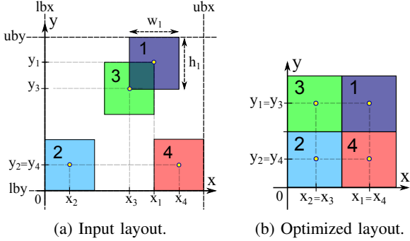
Fig. 3: Inequalities (3) ensure that no boxes will not displayed offscreen while inequalities (4) preserve the order of the coordinates w.r.t. initial layout. (a) Input layout and (b) result after layout arrangement (orthogonal ordering: x_{p_1} \leq x_{p_2} \leq x_{p_3} \leq x_{p_4} ; similarity for y case).
