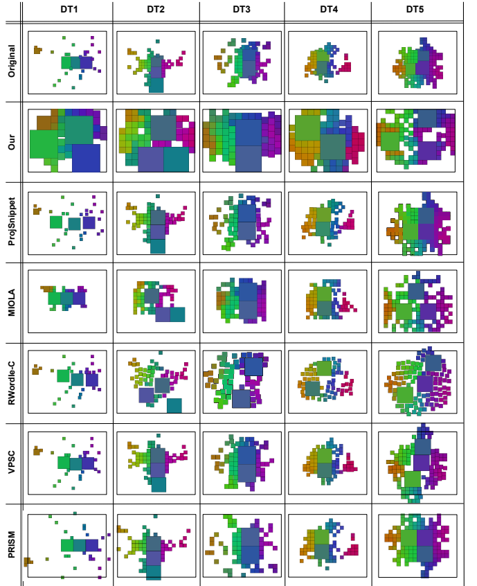
Fig. 6: Layouts produced by our approach, ProjSnippet, MIOLA, RWordle-C, VPSC and PRISM in 5 datasets.
