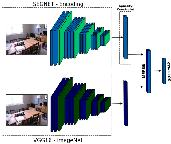
Fig. 2: Proposed architecture. Both SegNet (encoding) and VGG16 share the same architecture, and the final feature merges both of them.
