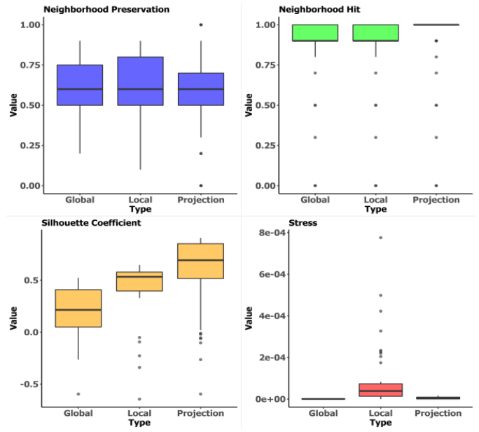
Fig. 6. Boxplots corresponding to the analysis of the iris dataset.
