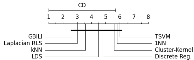
Fig. 4. Comparison of all classifiers against each other with the Nemenyi test.
