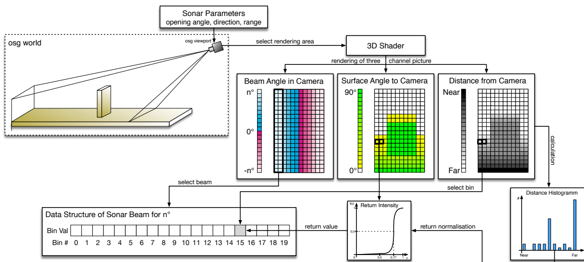
Fig. 1. A graphical representation of the individual steps to get from the OpenSceneGraph scene to a sonar beam data structure.
