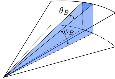
Fig. 2. Single sonar beam's geometry[6]
