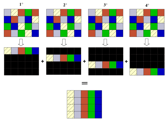
Fig. 2. Proposed method in PPM1 configuration with N = 80 , M = 20 , and k = 4 . For each subframe, only one set of pixels ( M/k = 5 pixels) receives light. The mirror pattern is the same for all subframes.
