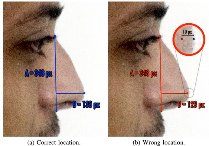
Fig. 9. A misplacement of only 10 pixels left of the correct tip location causes the Baum ratio to increase from 2.6 to 2.8. That would mean this nose’s tip is ideal, which is not correct.
