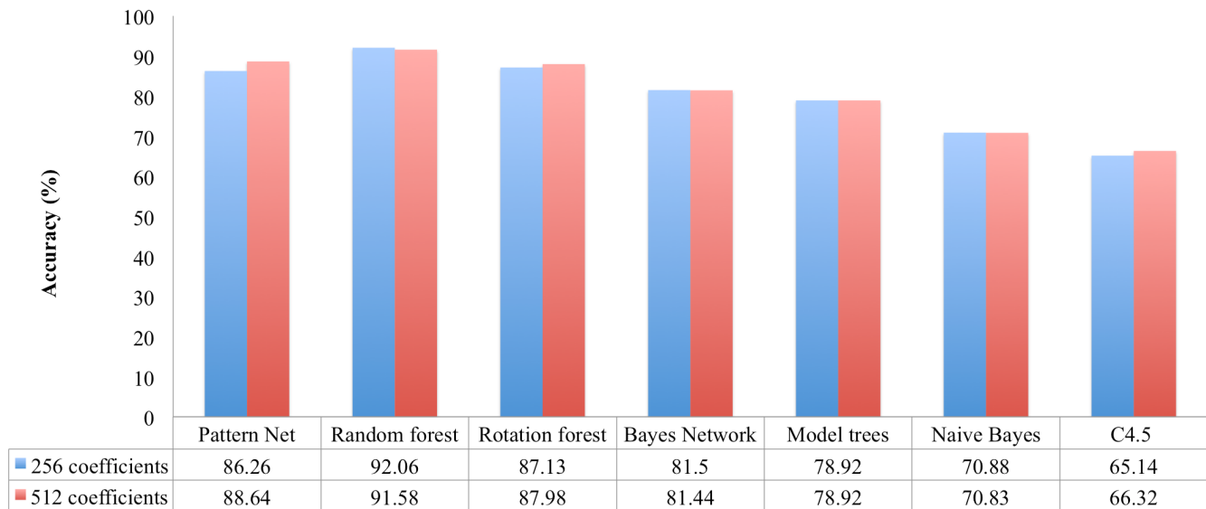
Fig. 4. Measure of Fourier descriptors accuracy. This figure aims to illustrate the influence of the symmetry property of Fourier transform through different classifier models.
