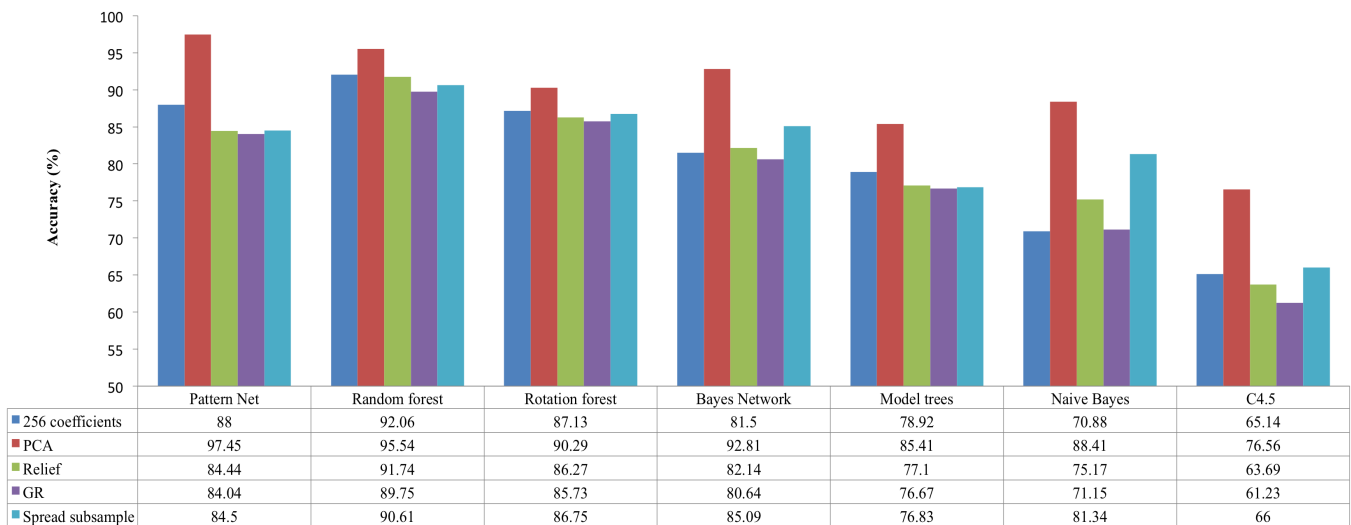
Fig. 5. Measure of accuracy of selected feature vectors. The feature selectors were applied over 256 Fourier descriptors.
