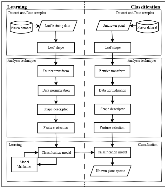
Fig. 2. Architecture of the leaf-based framework for plant classification
