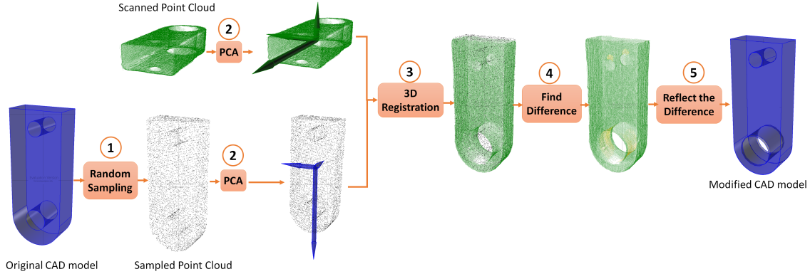
Figure 4. Method Steps: 1- Convert the 3D mesh or CAD model to point cloud. 2- Perform the principal component analysis for the two point clouds. 3- 3D registration. 4- Finding the difference. 5- Reflecting the changes to the 3D mesh or CAD model.
