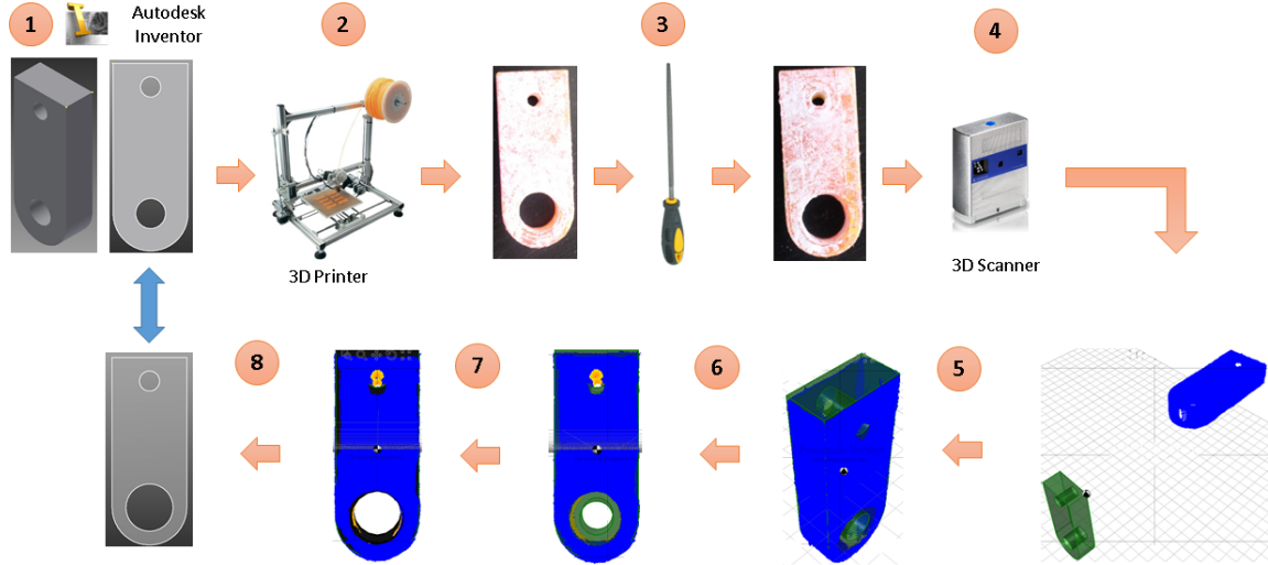
Figure 5. 3D printing experiment steps: 1- Draw the model in Autodesk inventor 2- Print the model using 3D printer 3- Using round file to expand the hole in the physical object 4- Scan the object using 3D scanner 5- 3D registration between the scan point cloud and the CAD model 6- Find and visualize the difference region (shown in yellow) 7- Reflect the changes by expanding the same region in the CAD model 8- Export the modified CAD model and import it back to Autodesk Inventor
