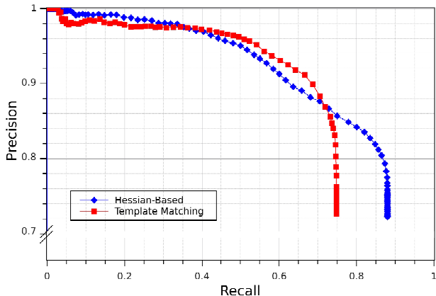
Fig. 5. Precision recall curves obtained for the proposed method (Hessian-based) and the TM.
