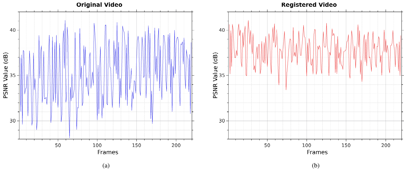
Fig. 4. PSNR metric processed over all the residual images from all consecutive video frames. (a) PSNR values before and (b) after registration.
