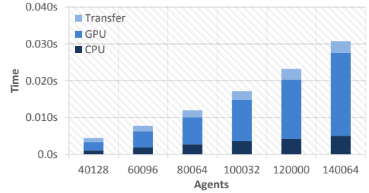
Figure 6: Total computational time of one iteration (Algorithm 1) on the Glob mesh. The time that the CPU is waiting for the GPU is accounted in the GPU processing time.
