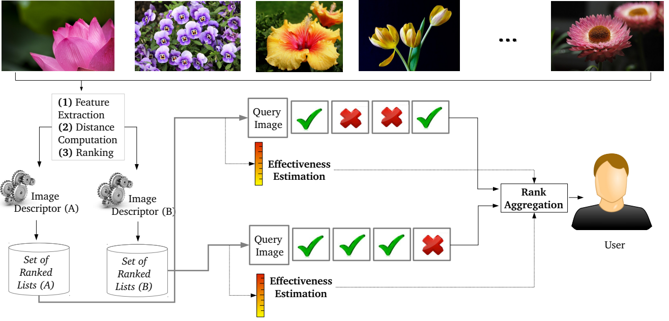
Fig. 2. General workflow of the use of unsupervised estimation measures for rank aggregation tasks.
