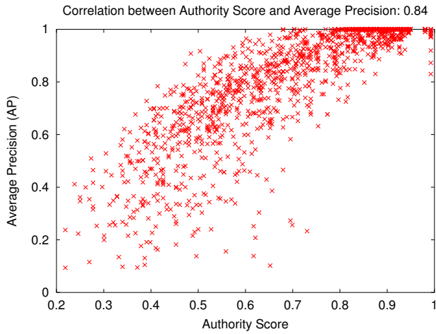
Fig. 3. Correlation Results between Authority Score and Average Precision, considering the CFD [24] shape descriptor.
