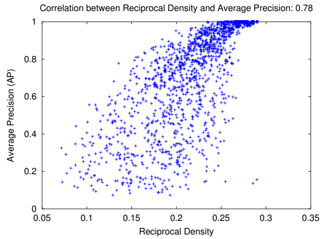
Fig. 6. Correlation Results between Reciprocal Density and Average Precision, considering the LAS [32] texture descriptor.
