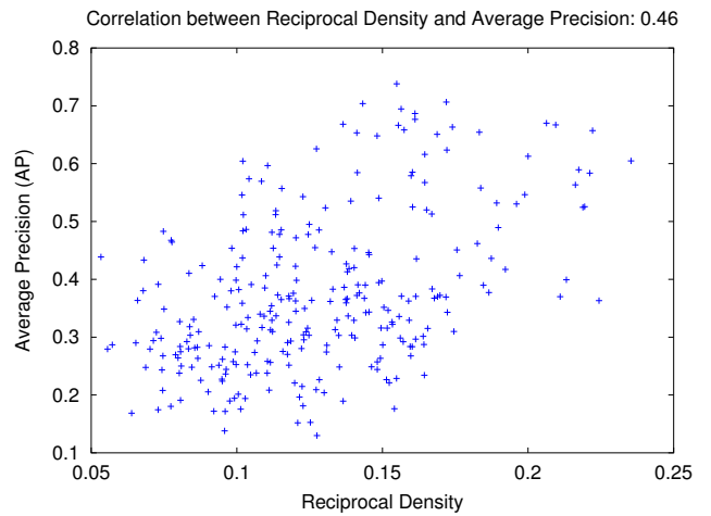
Fig. 8. Correlation Results between Reciprocal Density and Average Precision, considering the ACC [28] color descriptor.
