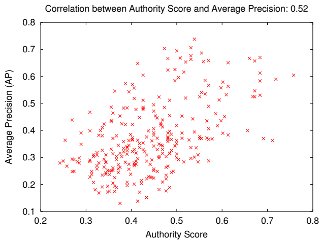
Fig. 7. Correlation Results between Authority Score and Average Precision, considering the ACC [28] color descriptor.
