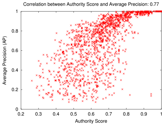
Fig. 5. Correlation Results between Authority Score and Average Precision, considering the LAS [32] texture descriptor.
