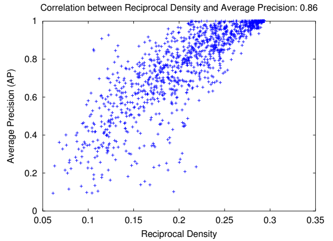
Fig. 4. Correlation Results between Reciprocal Density and Average Precision, considering the CFD [24] shape descriptor.
