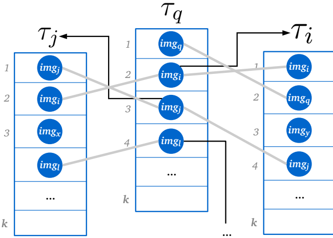
Fig. 1. Example of Authority Score [3] computation for the ranked list \tau_q obtained for image img_q . The images img_i, img_j represent k -nearest neighbors. The Authority Score is defined by the number of references among the k -nearest neighbors, represented by the edges, in gray.
