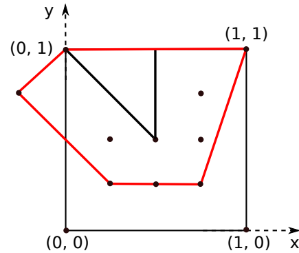
Fig. 6: Node with two adjacent links. The link to the upper-left node adds just one point to the control polygon that shapes the cell and not two points, like in Figure 4.
