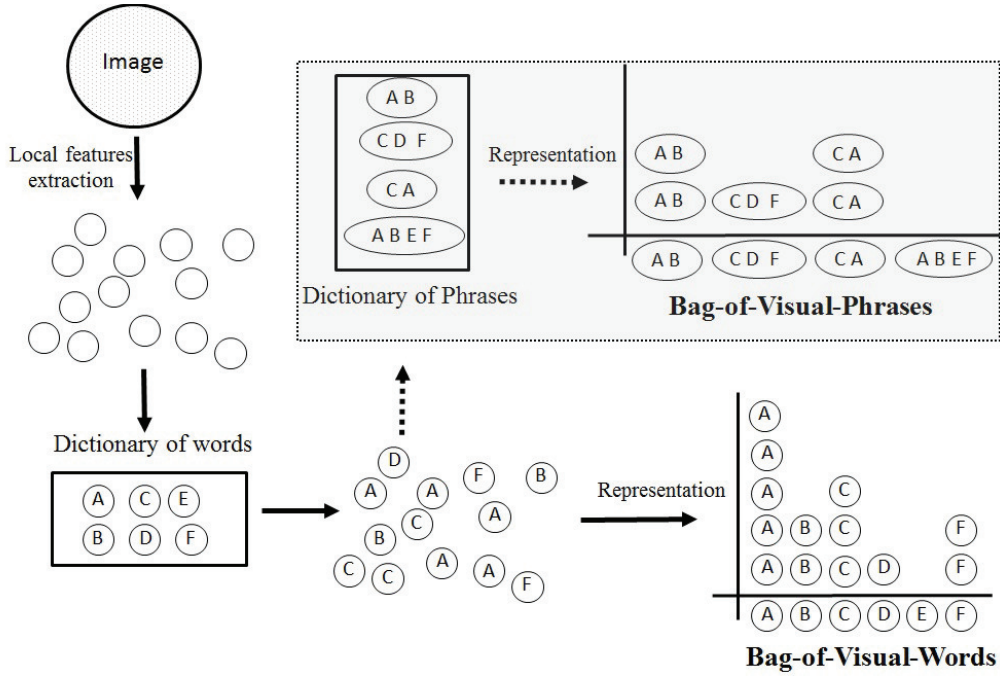
Figure 1. Scheme to represent an image in Bag-of-Visual-Word and Bag-of-Visual-Phrases.
