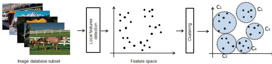
Figure 2. Process used to generate a visual dictionary. Initially, a keypoint detector is applied in a set of training images to detect representative local image points. The detected keypoints are represented by a descriptor that summarizes the information about the region around each keypoint. A dictionary can be built by clustering the keypoints detected.
