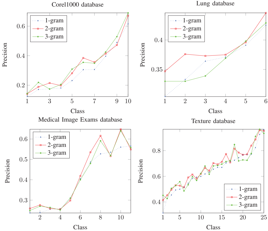
Figure 6. Precision values for each class of the evaluated databases.
