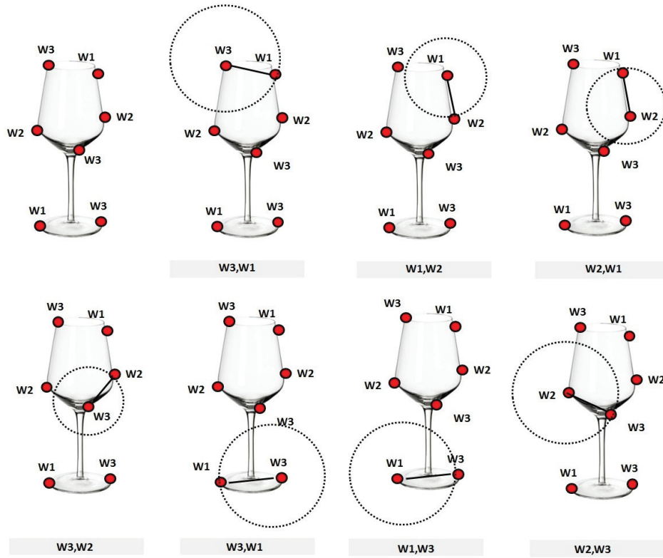
Figure 3. Example of the process used to extract 2-grams from an image. For each keypoint we look at its closest neighbor point. To extract n -grams from an image, with n > 2 , we just need to increase the number of nearest points.
