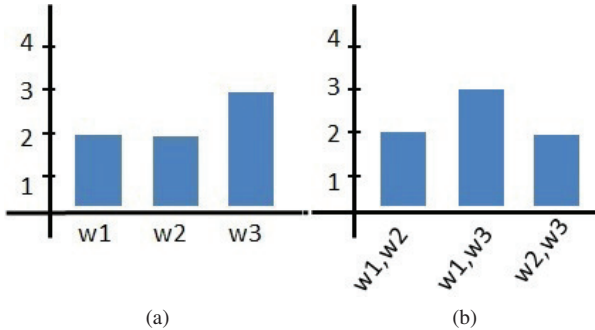
Figure 4. Representation of the image in fig. 3 by: (a) Bag-of-Visual-Words, (b) Bag-of-Visual-Phrase considering 2-gram phrases and the proposed dictionary.
