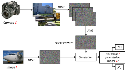
Fig. 2. Lukas et al. [9] approach.
