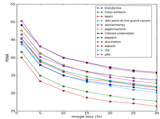
Fig. 9. PSNR values for reconstructed images versus percentage of deleted blocks.
