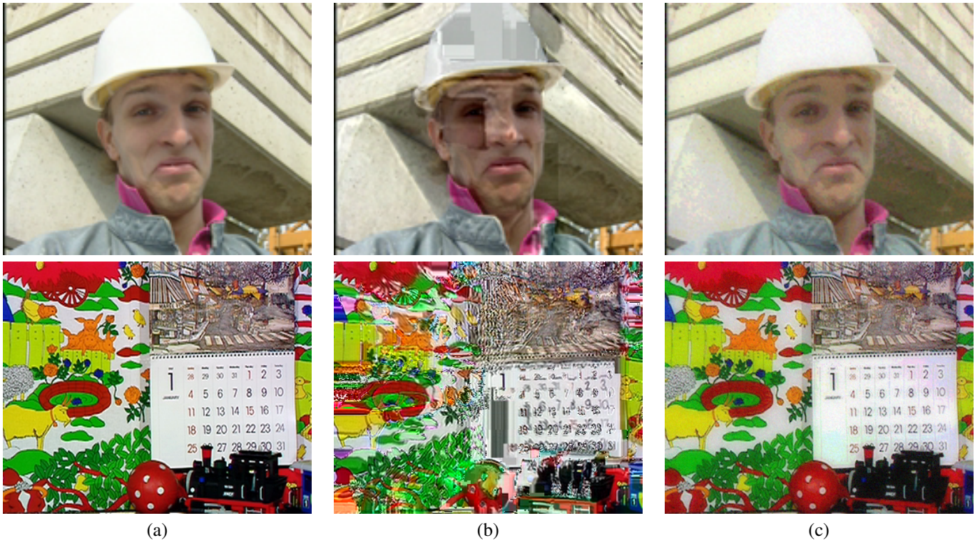
Fig. 10. Visual result of a reconstructed frame after a lossy transmission. (a) Original frames, (b) restored frames using default H.264 error concealment algorithm, (c) restored frames using the proposed algorithm.
