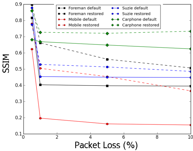
Fig. 11. SSIM values for reconstructed videos versus packet loss rate (PLR) values.
