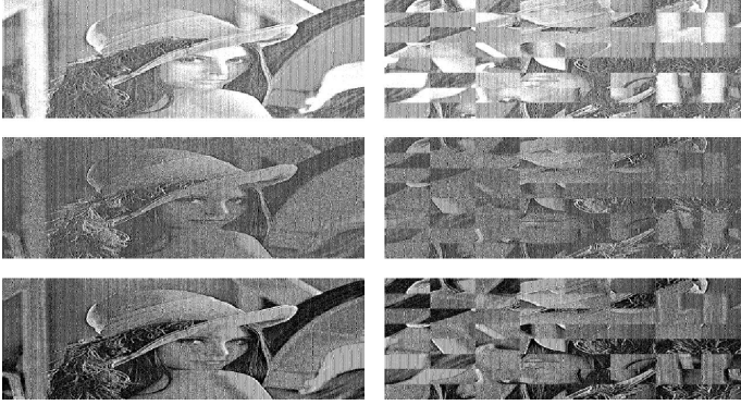
Fig. 4. Original dithered halftoned versions of each color channel of the image ‘‘Lena’’ (left) and the corresponding split-flip versions (right).
