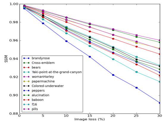
Fig. 8. SSIM values for reconstructed images versus percentage of deleted blocks.
