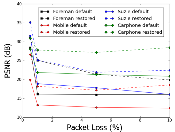
Fig. 12. PSNR values for reconstructed videos versus packet loss rate (PLR) values.
