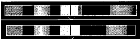
Figure 4: Examples of 1D simulated retinas.
