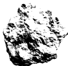
Figure 3: Fractal Rock.
