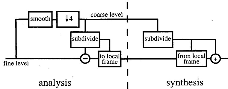
Figure 1: Synthesis and analysis diagrams for multiresolution surfaces.
