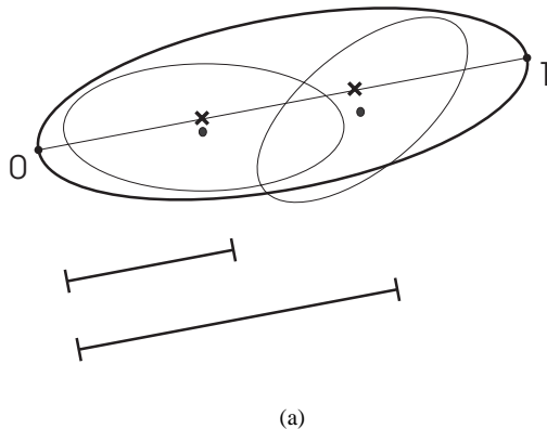
Figure 4: Projection of the centers of the ellipses contained in children nodes on the parameterized axis of the ellipse contained in the root node
