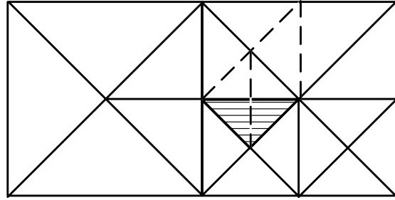
Figure 3: The basic refinement applied to the hatched triangle of a 2D AS triangulation. The dashed lines represent the three nucleus refinements.
