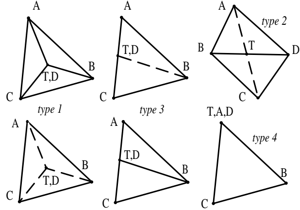
Figure 1: Possible projections of a tetrahedron with vertices A, B, C and D.
