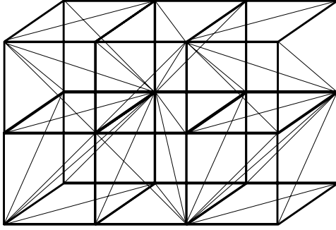
Figure 2: J1 triangulation of an array of 2x3 cubes.
