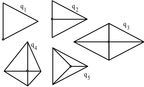
Figure 4: The 5 possible projections of AS triangulation tetrahedra for special directions.
