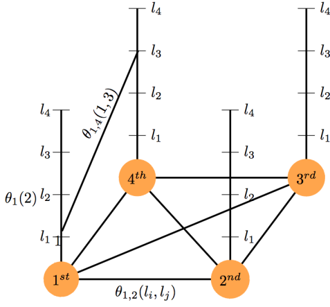
Fig. 4. Illustrative example (taken from [37]) of the MRF used when four targets are in the scene. Labels encode the set of targets in the scene, whereas the nodes correspond to the order that they will be imaged. Unary costs represent the angular differences between the current position of the camera and each target, whereas pairwise costs model the transition angles.
