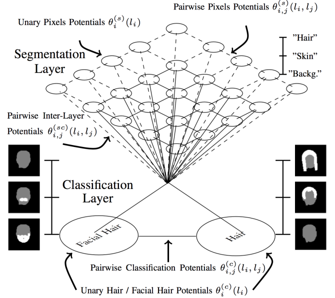
Fig. 7. Structure of a MRF (taken from [50]) that fuses the data appearance information (upper layer) to global constraints (bottom layer). During optimization, the network should converge into a balance point where the predominant labels at the segmentation level are biologically plausible and accord globally coherent facial hair / hair hypotheses (at the classification level).
