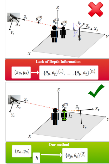
Fig. 3. Illustration (adapted from [36]) of the principal bottleneck of master-slave systems and the proposed strategy to address this problem. One image pixel (x_s, y_s) might correspond to multiple 3D positions in the scene, and consequently to different pan-tilt \{\theta_p, \theta_t\} values. Our work is based on the premise that human height h can be exploited to infer depth information and avoid the 2D \rightarrow 3D ambiguity.
