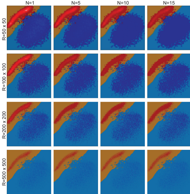
Fig. 3. The effect of varying both resolution R (rows) and number of minimum samples per pixel N (columns).
