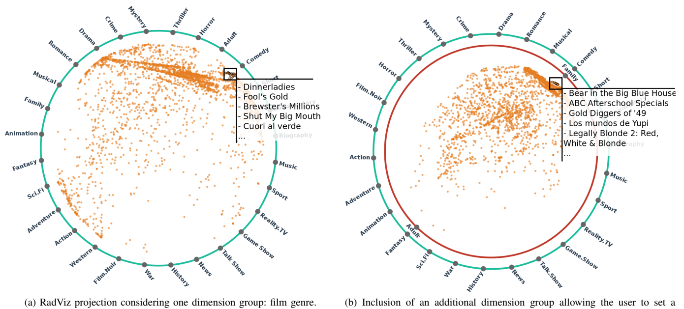
Fig. 6. Concentric RadViz with the IMDB-F film dataset.
