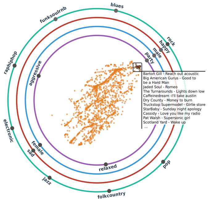
Fig. 5. Concentric RadViz with the Dortmund music dataset.
