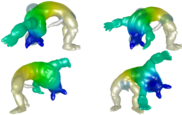
Fig. 3. Lagrange Polynomial weights
