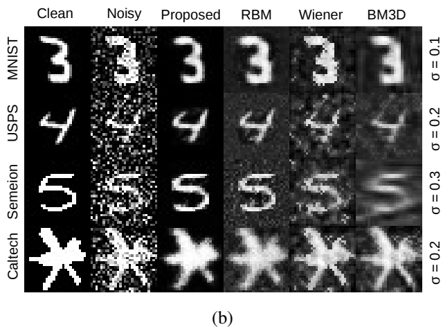
Fig. 4. Standard setting: (a) quantitative results over Caltech, MNIST, USPS, and Semeion datasets; and (b) qualitative results over MNIST, USPS, and Semeion datasets. Notice that \sigma denotes the variance of the Gaussian noise.
