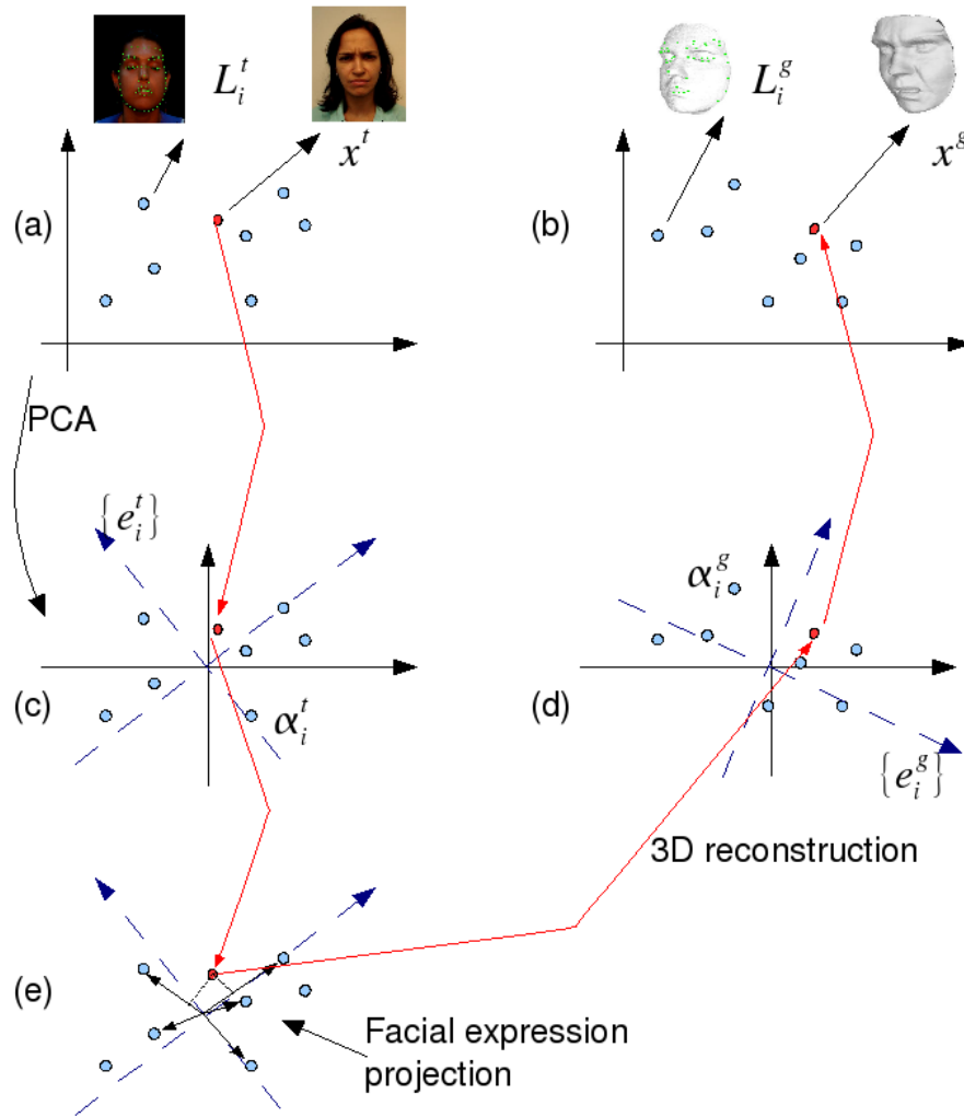
Figure 3. Texture and geometry spaces. x^t is an input texture face which undergoes a series of transformations through texture and geometry space until its geometry x^g is built.
