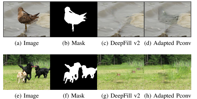
Fig. 3. Qualitative difference between inpainting performed by the previous method Adapted Pconv [17] (Subfigures 3d,3h) and the new one DeepFill v2 [27], [28] (Subfigures 3c,3g). Note how the DeepFill v2 method produces a more detailed erasure while sometimes producing an artifact (Subfigure 3g) on the image.
