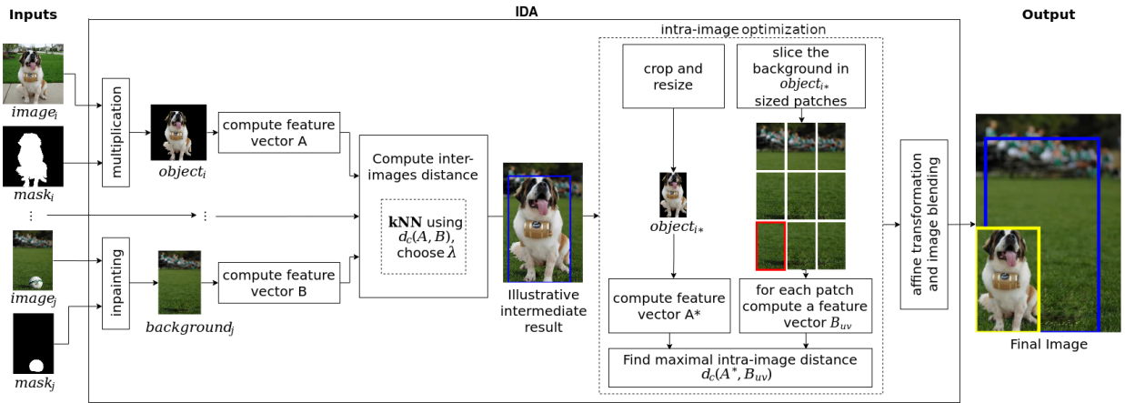
Fig. 1. Flowchart of the IDA technique. The first step is the computation of a background image for all the images of the inputted dataset; an object image is also computed; those images are used to produce feature vectors that can be compared using kNN with cosine similarity; \lambda stands for the criteria chosen, further details on Section III-B. Highlighted in blue is the intermediate bounding box of the object before the affine transformation. An intra-image optimization determines the translation of the object in the new background. Highlighted in red is the patch that produces the maximal distance intra-image in this example. Finally, for each pair of object_i and background_j , a final image is created using a linear combination of both. Highlighted in yellow is the final bounding box of the object.
