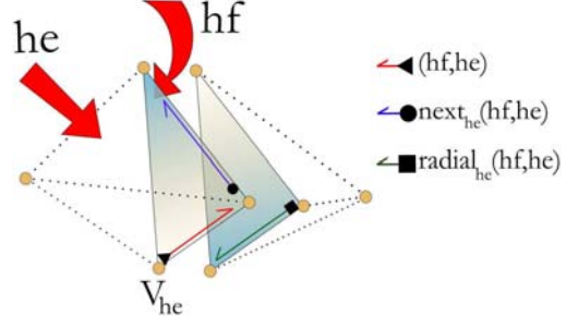
Figure 9. Radial half-edge.
