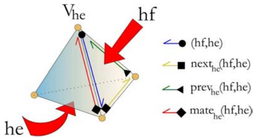
Figure 8. Mate half-edge.
