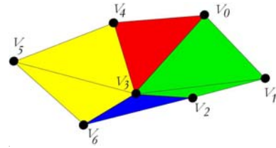
Figure 10. CHF level 1.
