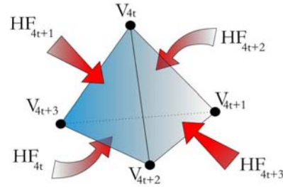
Figure 6. Insides of half-faces and vertices.
