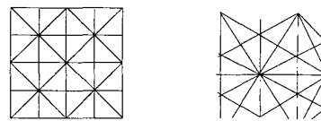
Figure 3: Laves tilings [4.8^2] and [4.6.12]
