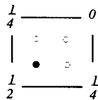
Figure 13: Mask for c_0 using dual quad-mesh refinement of the ZP subdivision scheme.
