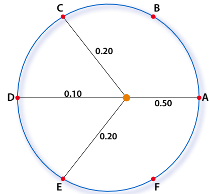
Fig. 2. Cancellation of forces in RadViz with class probabilities.
