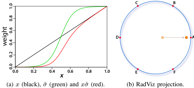
Fig. 3. RadViz with sigmoidal weighting: s = 15 and t = -0.5 .
