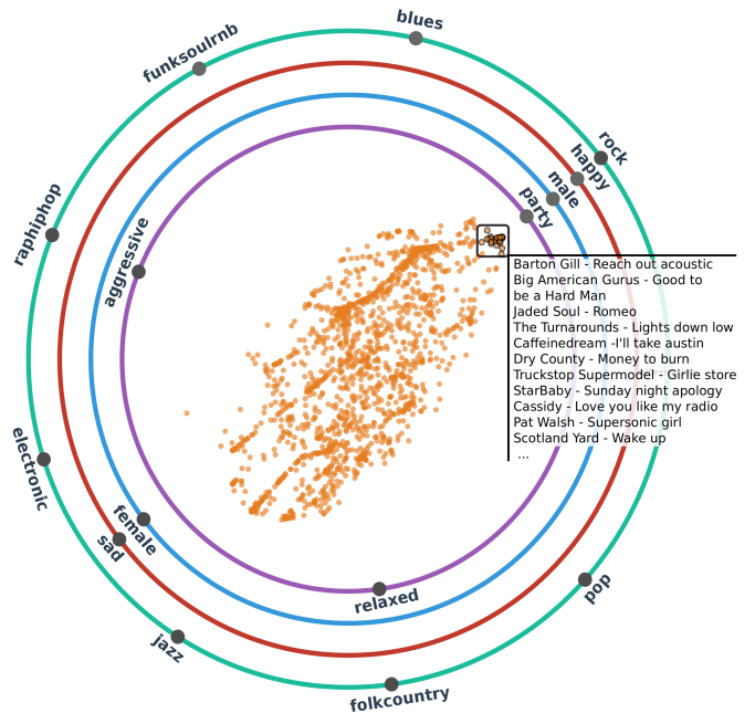
Fig. 5. Concentric RadViz with the Dortmund music dataset.
