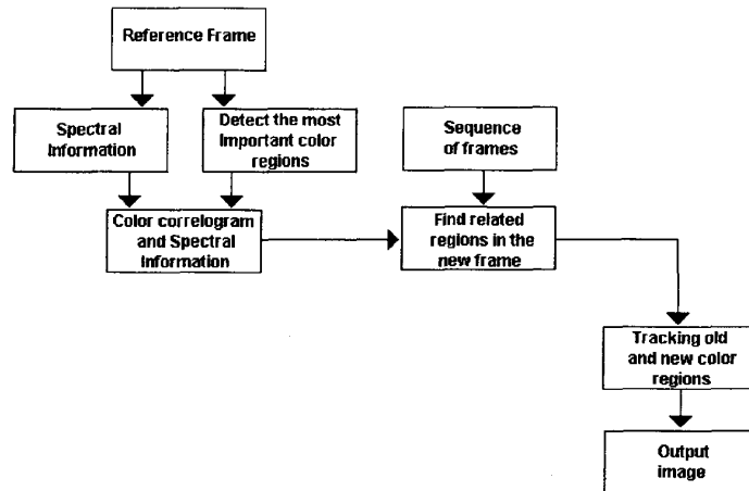
Figure 6: Visual Attention Model Diagram
