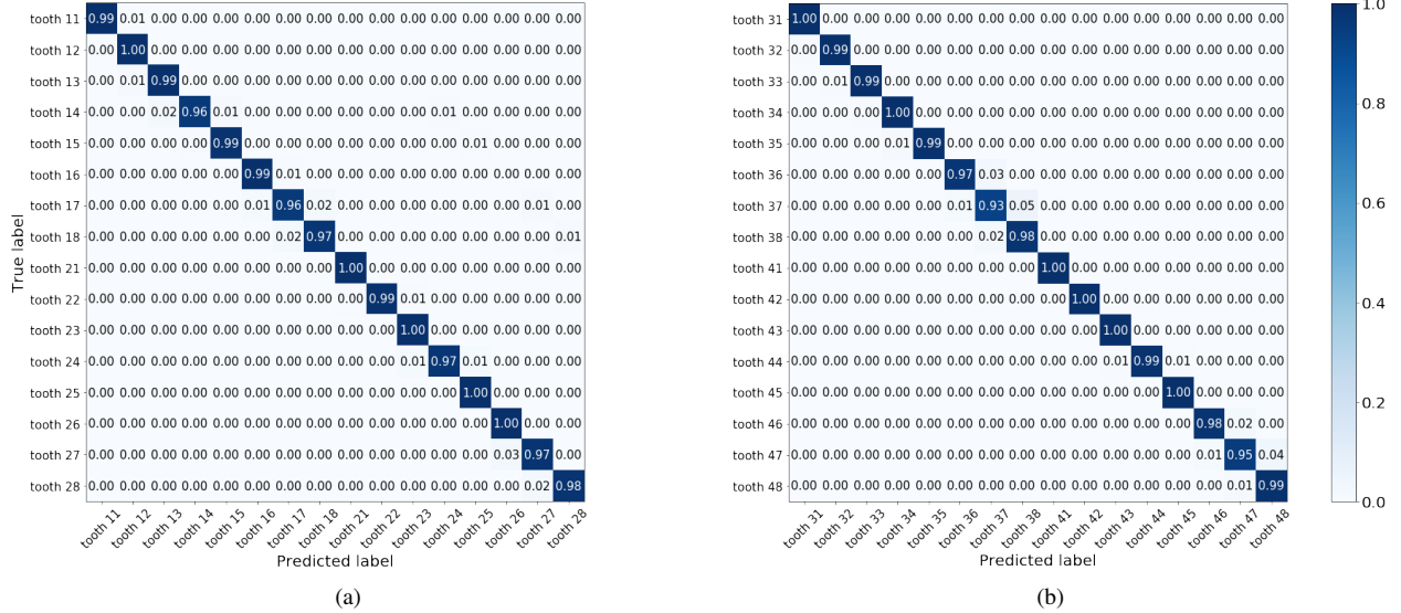
Fig. 3. Confusion matrices of the average results of the PANet architecture split into 2 parts: (a) superior dental arch, (b) inferior dental arch.
