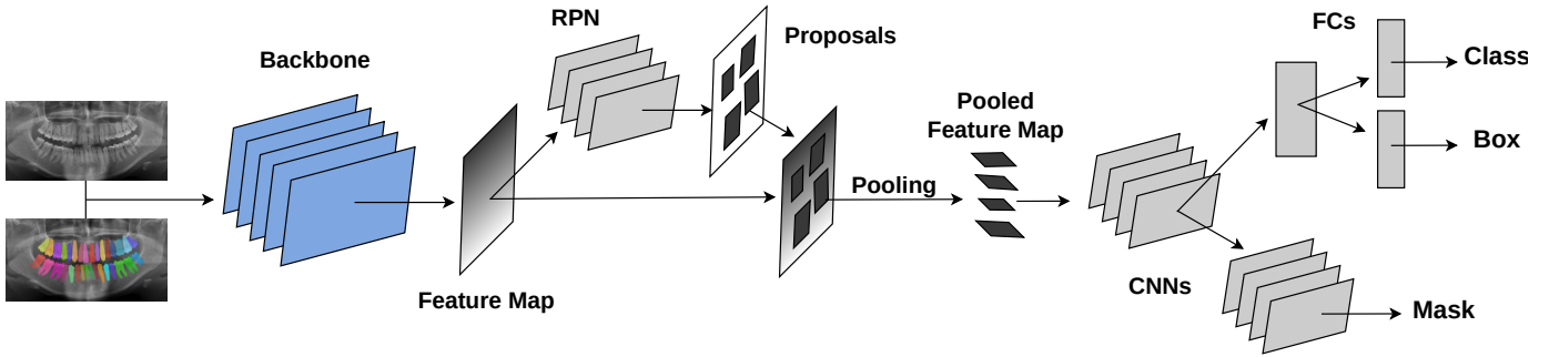
Fig. 2. General structure of an end-to-end instance segmentation network based on a two-stage detector.
