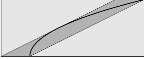
Figure 3: Zonotope approximation of a parabola segment.
