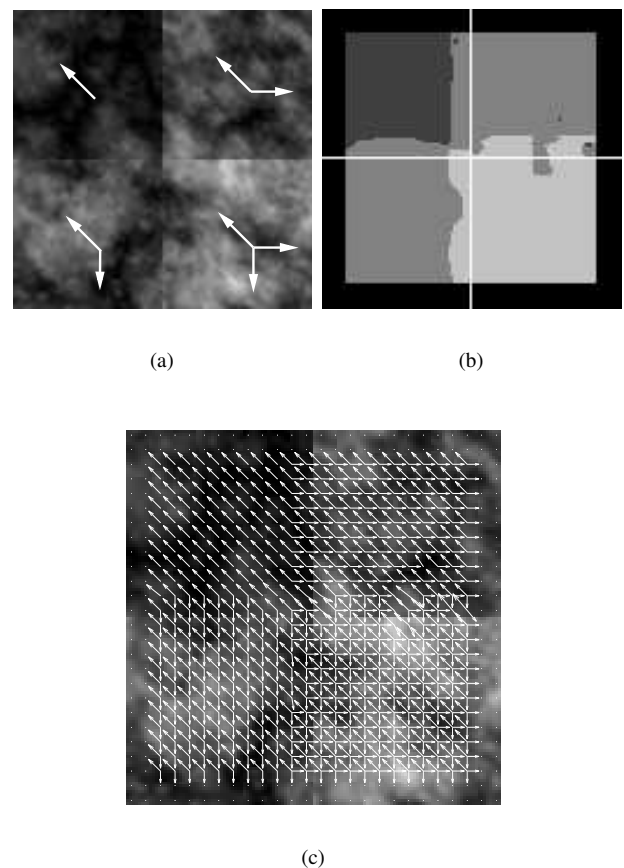
Figure 3. Synthetic example for estimation of one to three transparent superimposed motions.
